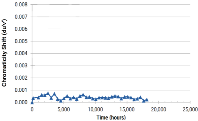
R1 Colour Shift Graph
